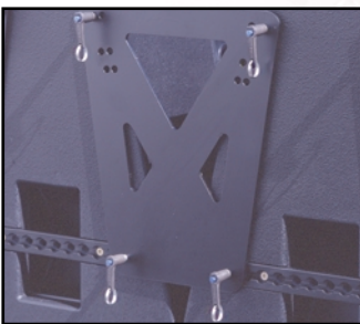
Rigid interconnect brackets with load rated, quick release pins offering multiple angles
